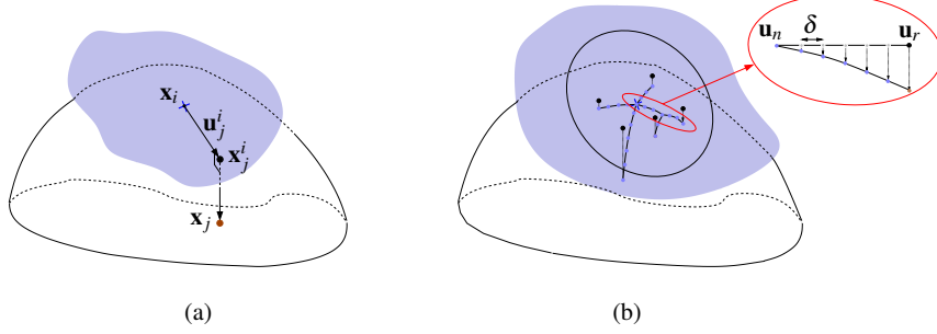
Fig. 2 (a) A chart C_i implements a mapping \mathbf{x}_j = \psi_i(\mathbf{u}_j^i) between the tangent space at \mathbf{x}_i and the manifold. (b) Growing a RRT on the manifold from a single chart. Black dots are the samples thrown in the tangent space and blue dots are points on the manifold forming the RRT branches. The inset shows the process of generating a branch by linear interpolation in the tangent space with steps of size \delta and successive projection.
