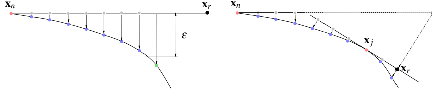
Fig. 4 RRT extension on a one-dimensional cut. The RRT is extended towards x_r , the randomly selected point, from x_n , the closest point already in the tree. In this case, x_n is the center of a chart. When the extension reaches a point (the green dot) where the error with respect to the chart at x_n is larger than \epsilon , a new chart is created from the previous node already in the tree and x_r is projected to the new chart. Then, the RRT extension continues in the new chart until the projected x_r is reached.
