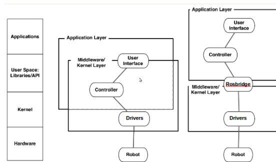
Fig. 1: Recreating traditional abstraction layers in robotics with rosbriidge. As depicted at left, software development depends on well-established layers of abstraction. Developers and engineers working at each layer possess very different skill sets, but the enterprise succeeds due to well-defined abstractions and interfaces. At present, roboticists must deal with all of these layers at once, limited by both their own skills and by the unwieldiness inherent in poorly-abstracted systems (center). At right, rosbriidge attempts to establish a more clear abstraction boundary to address this problem.
